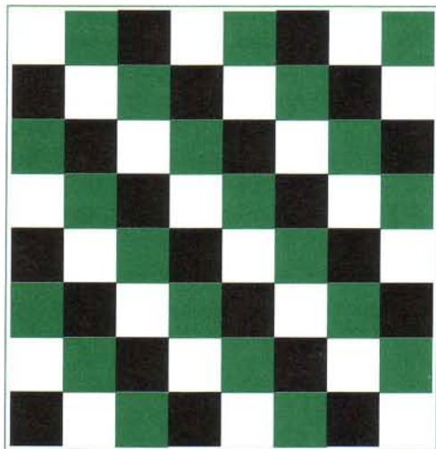
FIGURE 7 Coloring the Squares of the Standard Checkerboard with Opposite Squares Removed with Three Colors.
