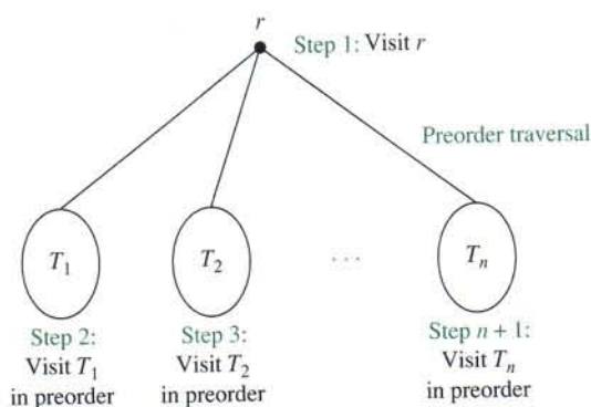
FIGURE 2 Preorder Traversal.
