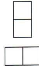
FIGURE 3 Two Dominoes.
