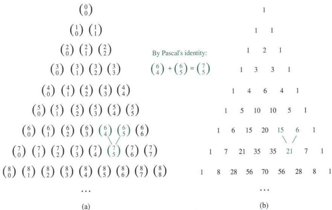
FIGURE 1 Pascal's Triangle.
