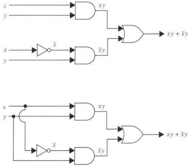
FIGURE 3 Two Ways to Draw the Same Circuit.
