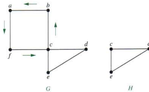
FIGURE 5 Constructing an Euler Circuit in G .
