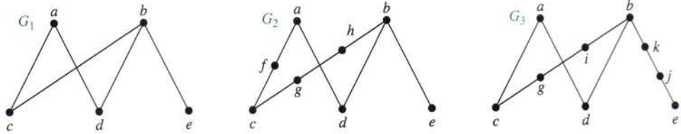
FIGURE 12 Homeomorphic Graphs.
