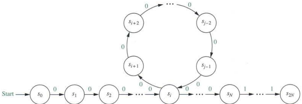
FIGURE 6 The Path Produced by 0^N 1^N .
