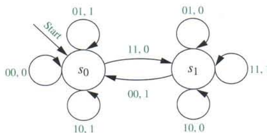
FIGURE 5 A Finite-State Machine for Addition.
