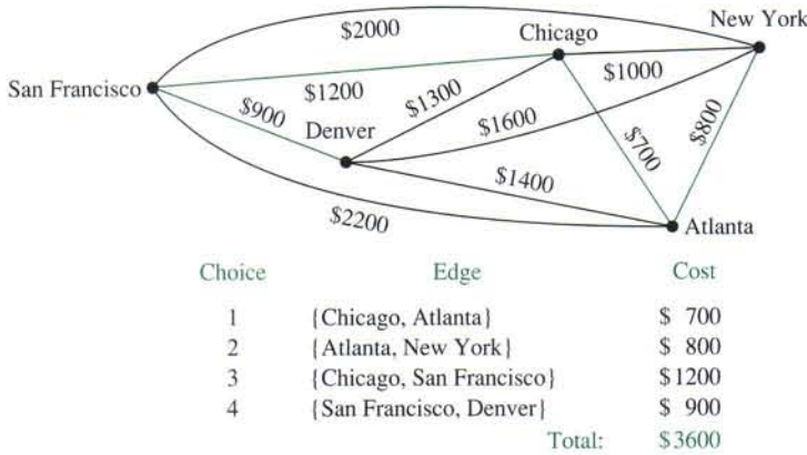
FIGURE 2 A Minimum Spanning Tree for the Weighted Graph in Figure 1.
