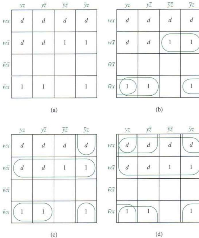
FIGURE 11 The K-map for F Showing Its Don't Care Positions.
