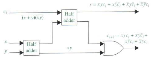
FIGURE 9 A Full Adder.
