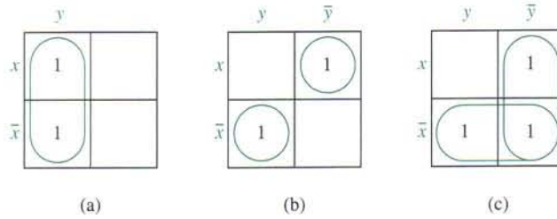
FIGURE 4 Simplifying the Sum-of-Products Expansion from Example 2.
