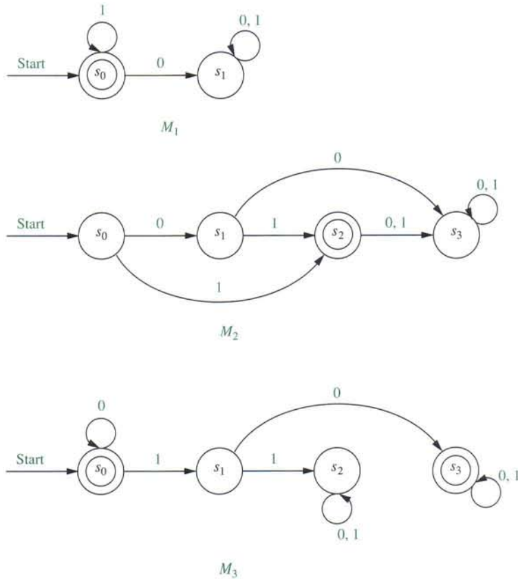
FIGURE 2 Some Finite-State Automata.
