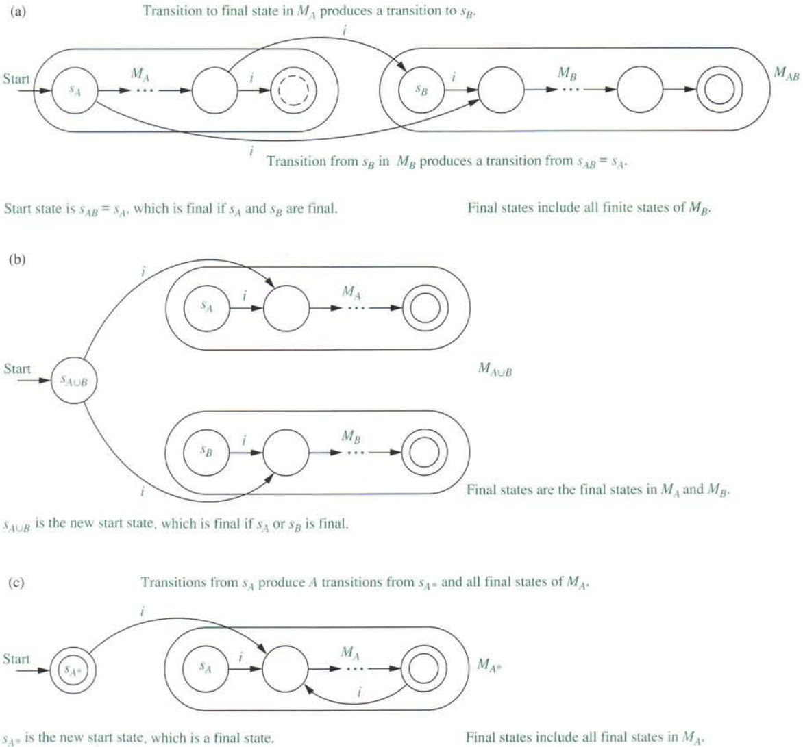
FIGURE 2 Building Automata to Recognize Concatenations, Unions, and Kleene Closures.
