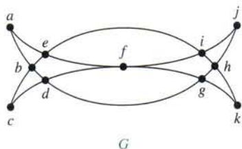
FIGURE 6 Mohammed's Scimitars.
