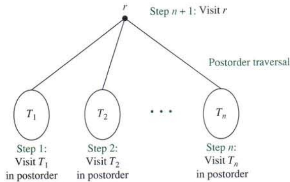
FIGURE 7 Postorder Traversal.
