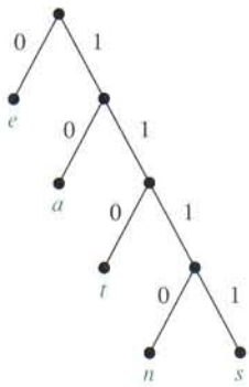
FIGURE 5 The Binary Tree with a Prefix Code.
