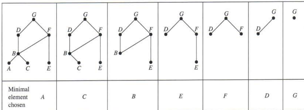
FIGURE 11 A Topological Sort of the Tasks.
