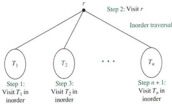
FIGURE 5 Inorder Traversal.
