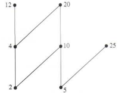
FIGURE 5 The Hasse Diagram of a Poset.
