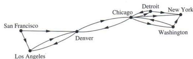
FIGURE 4 A Communications Network with One-Way Communications Links.
