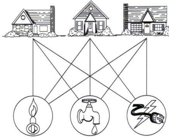
FIGURE 1 Three Houses and Three Utilities.
