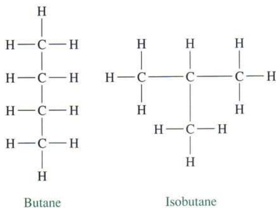
FIGURE 9 The Two Isomers of Butane.
